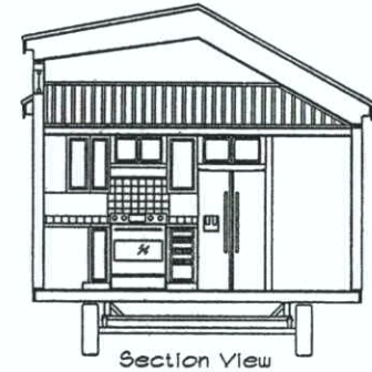
Section View
